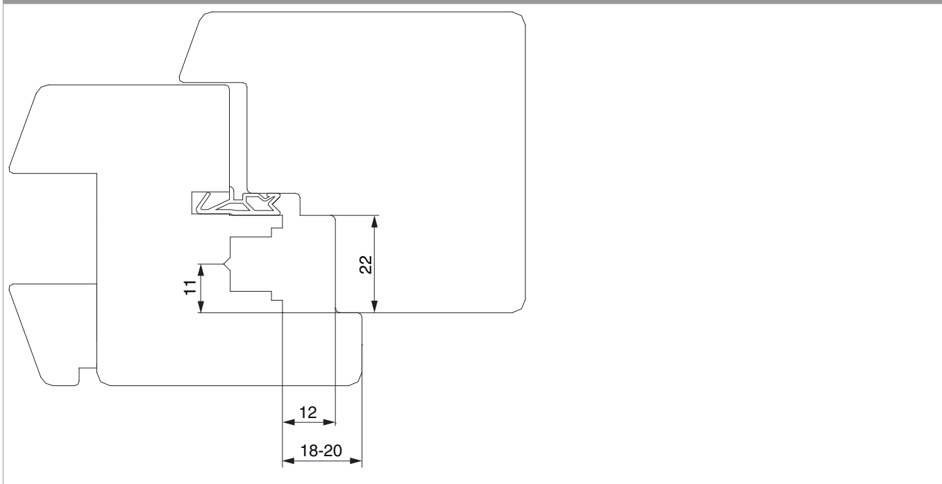
A12 PB22 - 1 anta
