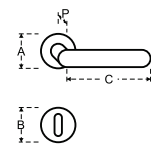
Maniglia con rosetta e bocchetta Handle with rose and lock profile
